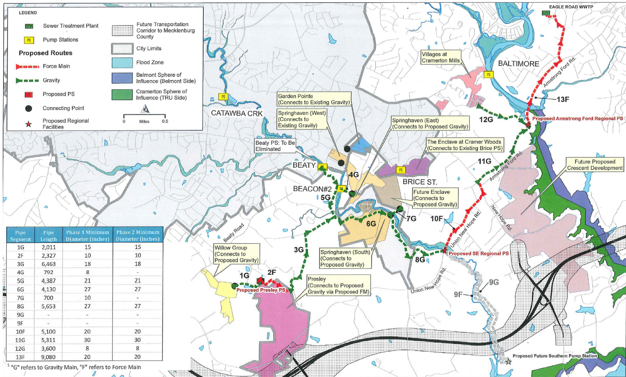
SOUTHEAST REGION TO EAGLE ROAD WWTP (PHASED APPROACH) FIGURE 5-2 - ALTERNATIVE 2
